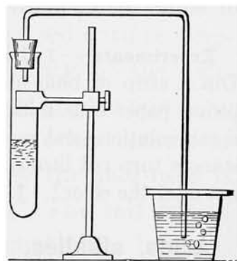
FIG. 7. — Apparatus for testing for carbon dioxide.
